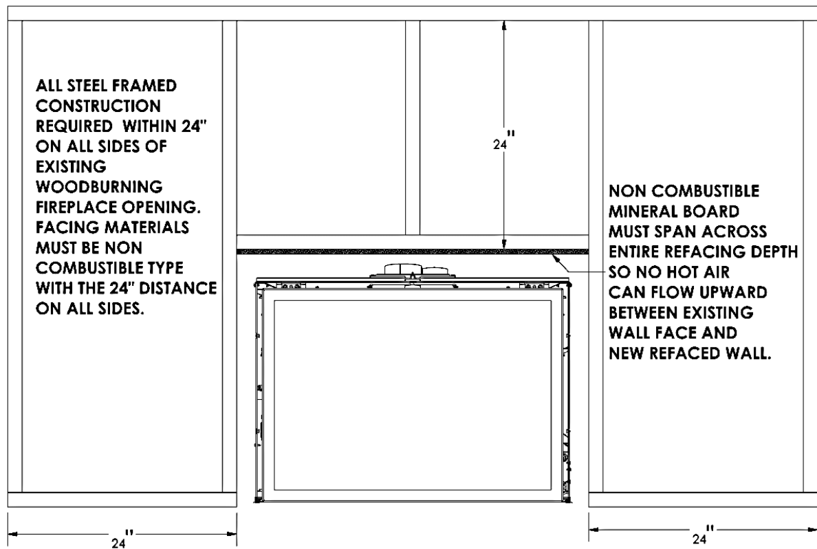
Figure 3-5 Re-facing Information
