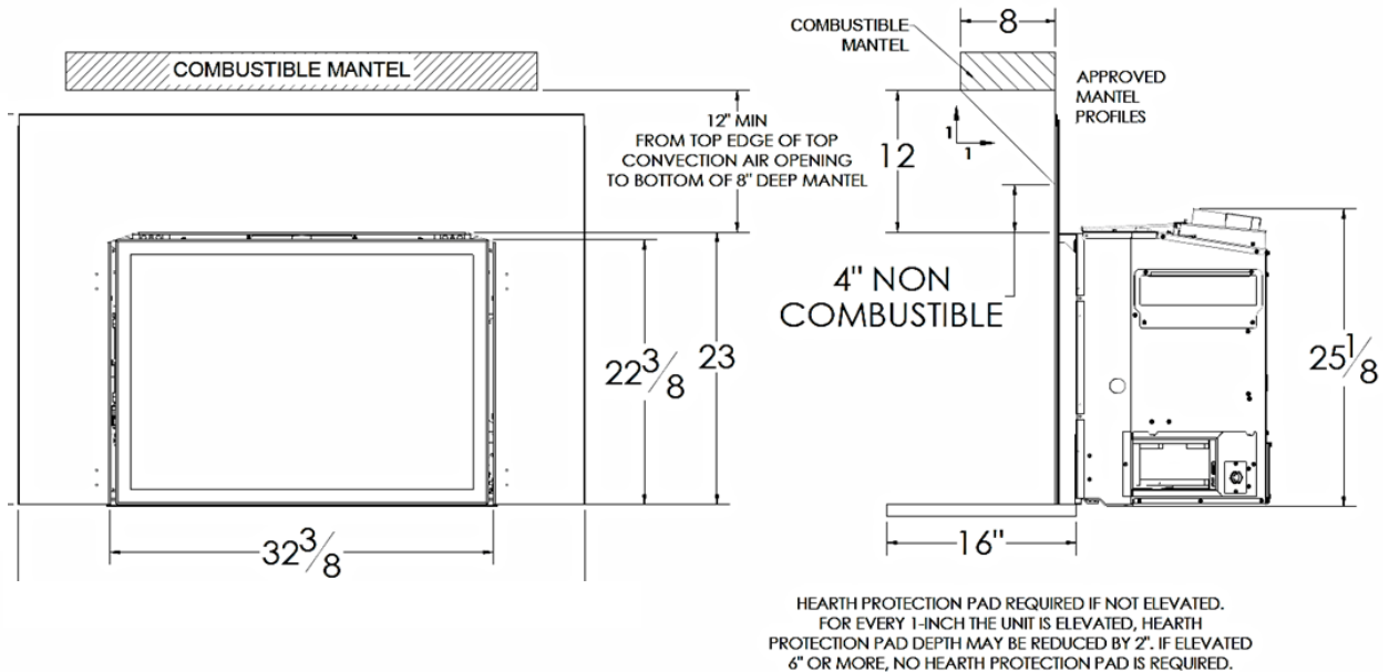
Mantel Clearances
