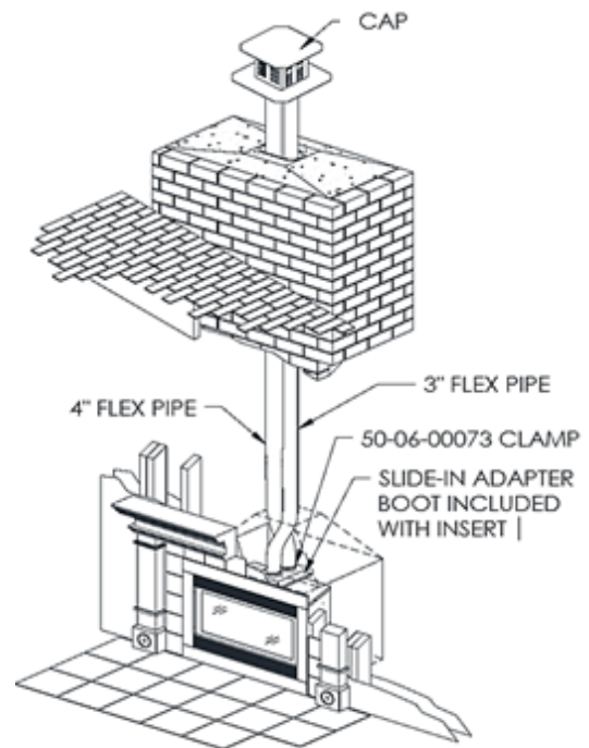
Vent System
